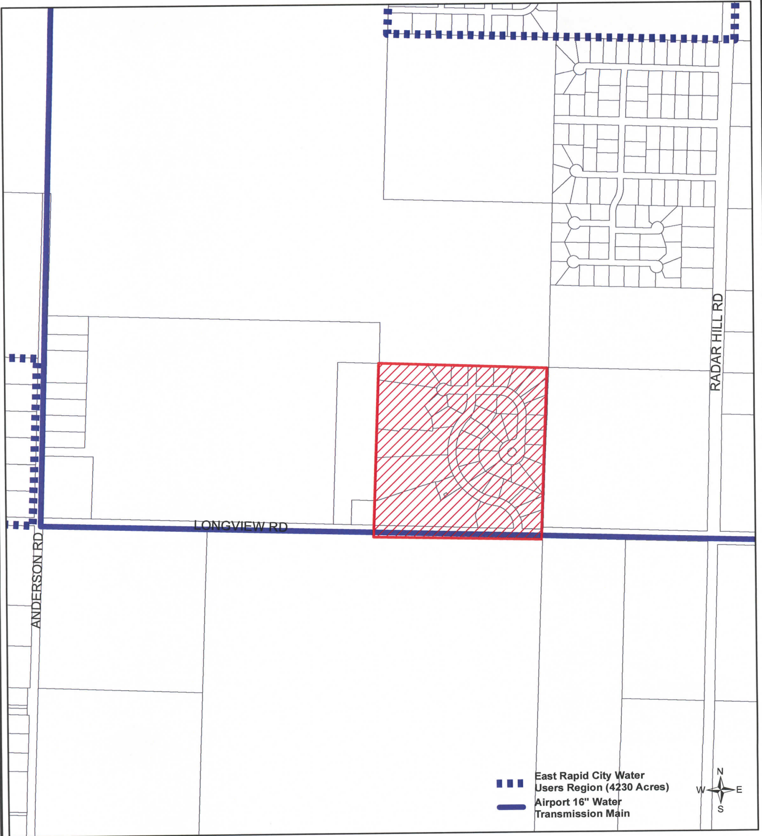
EAST RAPID CITY WATER EXPANSION PROJECT NO. 14-2198/CIP 50964.F Mesa View Estates Subdivision, Radar Hill Road and Morris Lane Water Extensions
