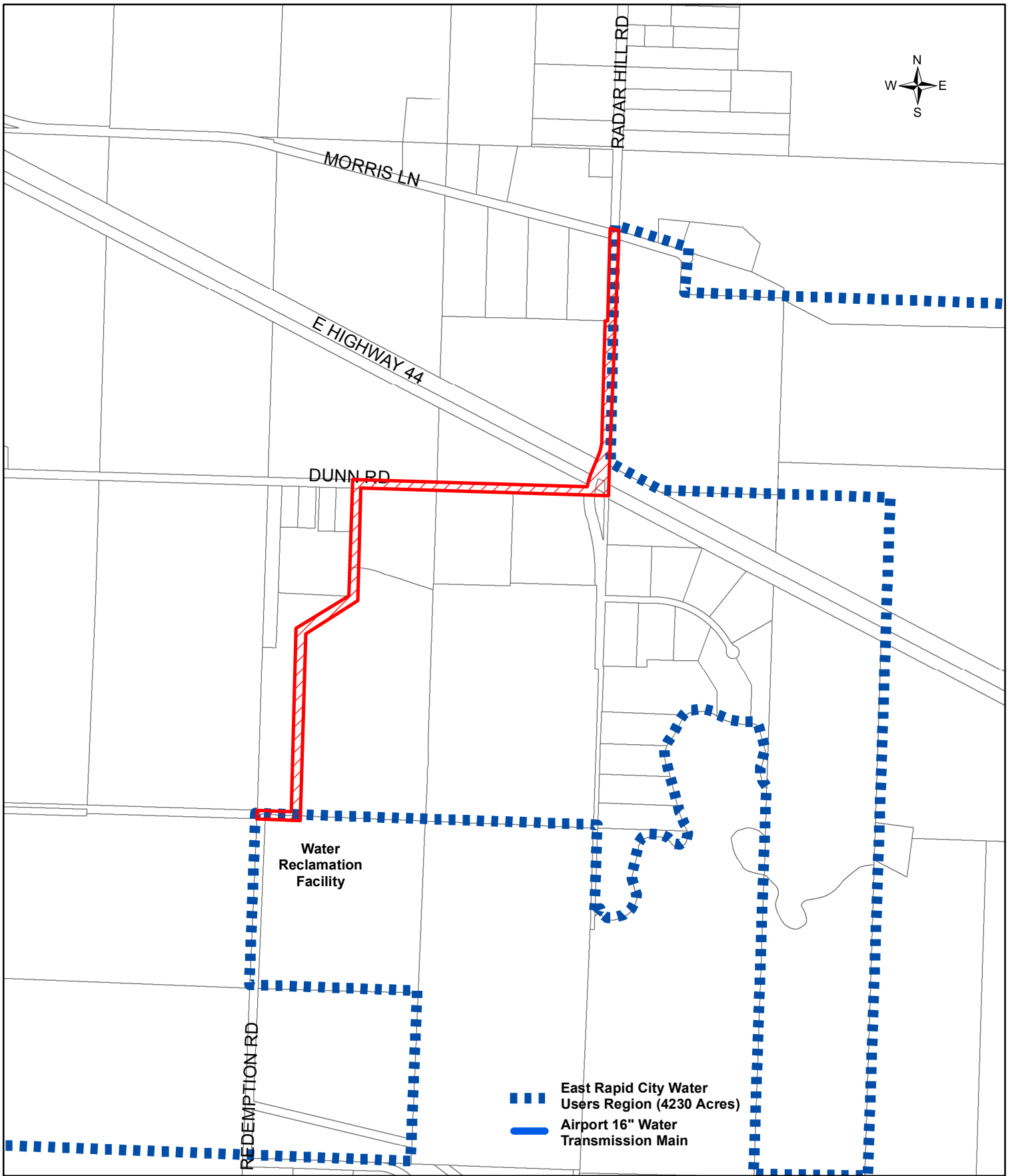
EAST RAPID CITY WATER EXPANSION Water Reclamation Facility Water Main Transmission Extension, Project No. 14-2196 / CIP No. 50964.D
