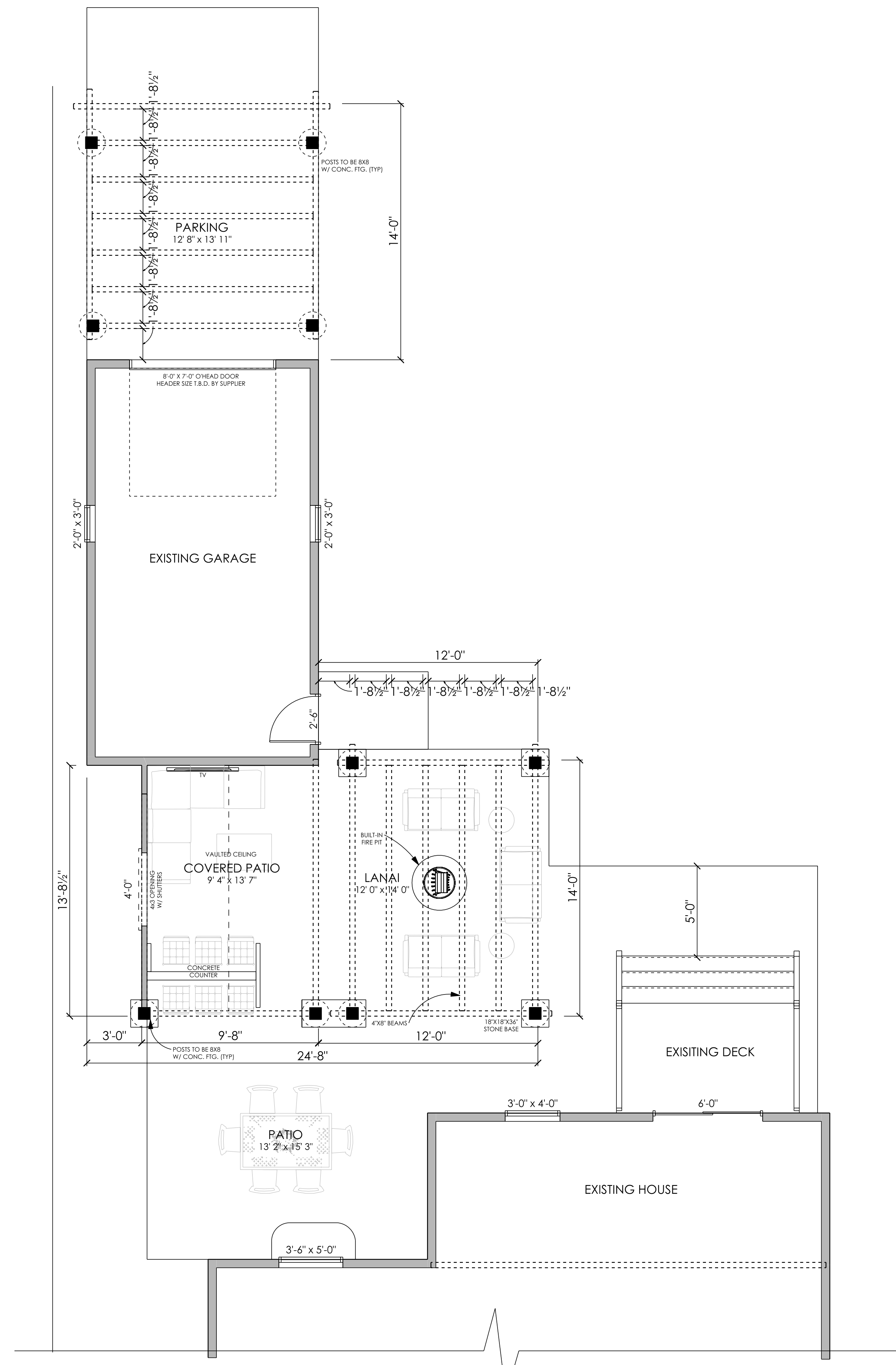
MAIN FLOOR PLAN SCALE: 1/4" = 1'
