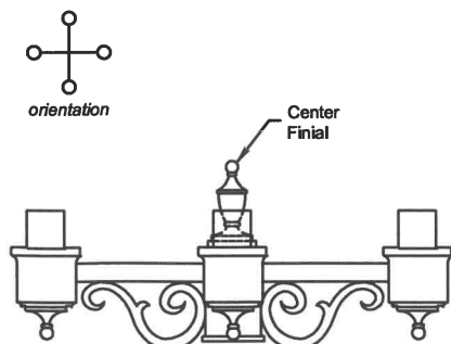
CSC30/4 (four at 90°)
