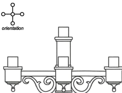
CSC30/4T (four at 90° w/ one at center)
