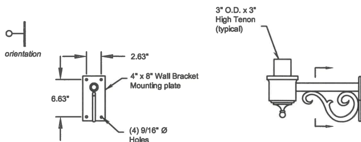
CSWB (one way wall mount)
